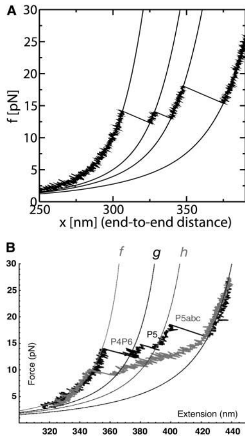
FIGURE 15 Comparison of FECs between model and experiments. (A) Numerical simulations of the pulling process at r = 4 pN/s for a three-domain RNA molecule. Simulations have been done with the effective model Eq. 36 without refolding. Domains are characterized by the following parameters: Domain 1, \bar{x}_1^{(1)} = 2.5 nm, \bar{B}^{(1)} \ln(k_0^{(1)}) = 8.5 k_B T ; Domain 2, \bar{x}_1^{(2)} = 2.5 nm, \bar{B}^{(2)} \ln(k_0^{(2)}) = 8 k_B T ; and Domain 3, \bar{x}_1^{(3)} = 1.7 nm, \bar{B}^{(3)} \ln(k_0^{(3)}) = 8.5 k_B T , where the super-index refers to the index of the domain. The solid lines correspond to the WLC force-extension curves. (B) Experimental FEC for the P4–P6 domain obtained by Onoa et al. (2003). The solid lines correspond to WLC curves for the handles linked to the RNA molecule. (Note that the lower curve corresponds to a refolding process we do not consider here.) Figure taken from Onoa et al. (2003).
