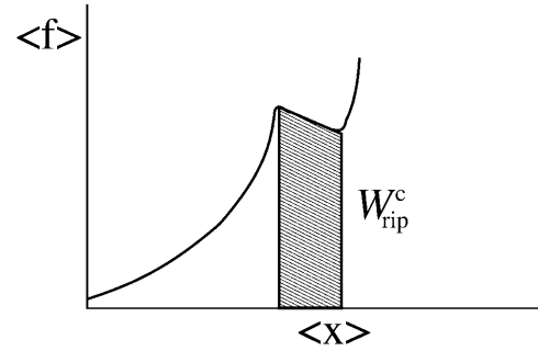
FIGURE 4 The shadow area under the TFEC along the transition corresponds to the quasistatic work W_{\text{rip}}^c (schematic representation).
