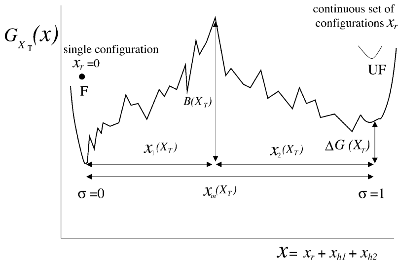
FIGURE 2 Schematic representation of the free-energy landscape, G_{X_T}(x) , for the whole system at temperature below the melting temperature, for X_T < X_T^c (where X_T^c is the value of X_T , in which both states F and UF are equiprobable) and normal ionic conditions. For this set of conditions, the stable state is the folded one. In this figure we represent all the parameters characterizing the two-states model. We also show the relevant configurations in the F and UF states along the reaction coordinate x_r : the F state is characterized by a single configuration x_r = 0 , whereas the UF state is represented by a continuous set of values of x_r . We use the label \sigma = 0 for the F state and \sigma = 1 for the UF state.
