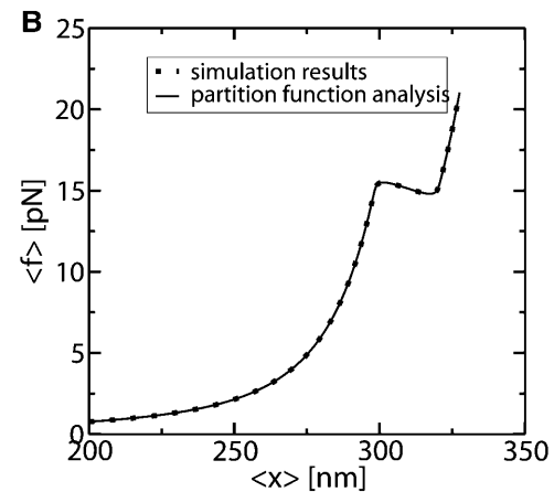
FIGURE 3 (A) Different contributions to the reversible work obtained from the partition function analysis: W_T^{\text{rev}} , W_h^{\text{rev}} , W_b^{\text{rev}} , and W_r^{\text{rev}} as a function of X_T . Note that the smallest contribution to the total work comes from the RNA molecule. (B) The continuous line corresponds to the results obtained from the numerical computation of the TFEC. It is also shown that the TFEC is obtained by averaging over 1000 different trajectories, as explained in Simulation of a Pulling Experiment. The pulling is carried out at an approximate loading rate of 0.5 pN/s, slow enough to generate a quasistatic process. One can observe that both curves agree.
